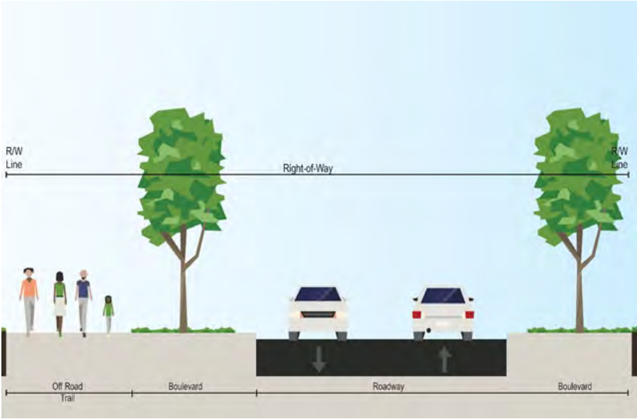
Figure 5-9: Off-Road Trail with Boulevard off Roadway
