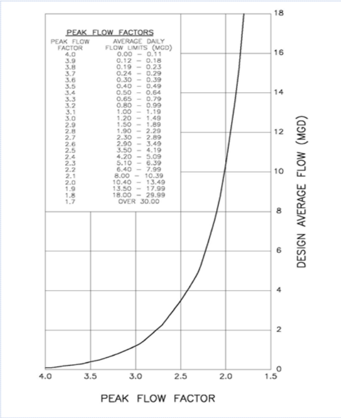
Figure 7-1: Peak Flows
