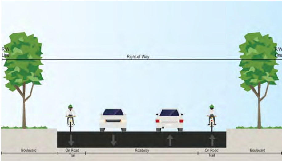
Figure 5-11: On Road Trail on Roadway with Boulevard
